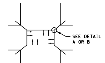
SUSPENDED BOX
