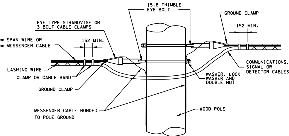
ALTERNATE CABLE CONTINUATION-SEPARATE MESSENGER CABLE
