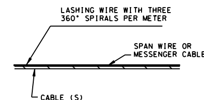
TYPICAL LASHING DETAIL
