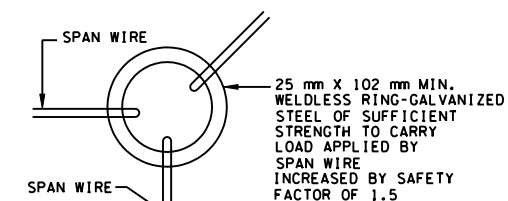
DETAIL A TENSION RING (TYP.)
