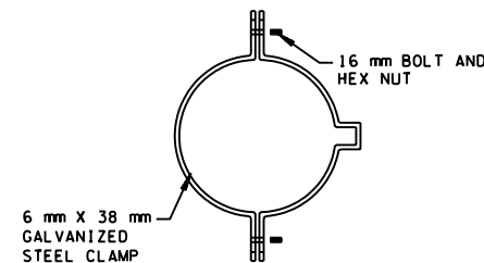
SPLIT CLAMP
