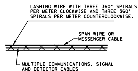
DOUBLE LASHING DETAIL
