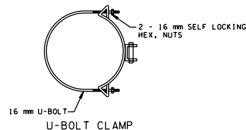
U-BOLT CLAMP
