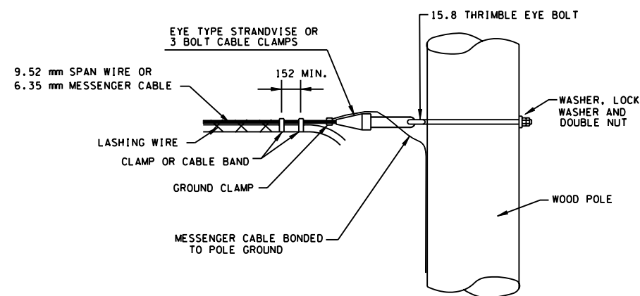
TYPICAL POLE ATTACHMENT DETAIL FOR MESSENGER DEAD END
