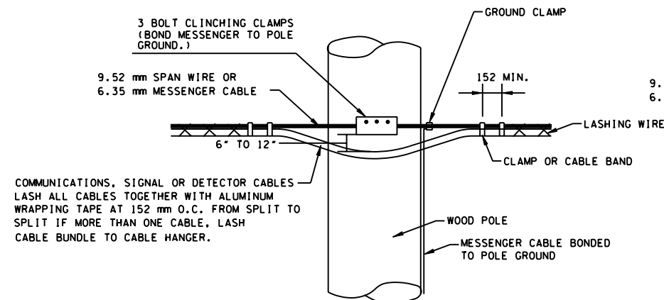
TYPICAL CABLE CONTINUATION-SAME MESSENGER CABLE
