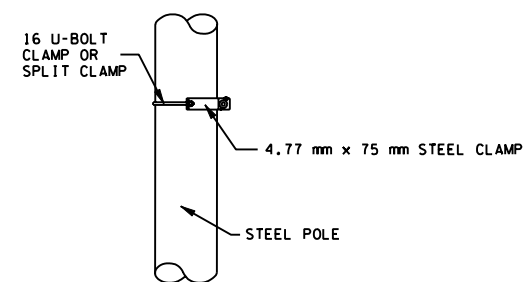
TYPICAL POLE ATTACHMENT FOR STEEL POLE
