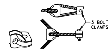
DETAIL B STRAND CONNECTOR (ALT.)
